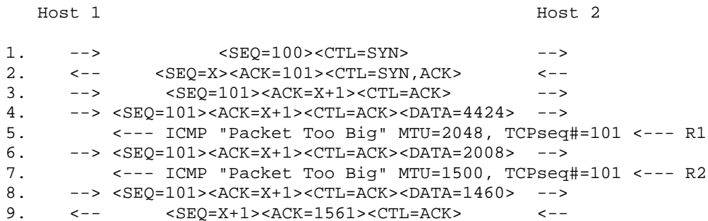
Figure 2: Normal operation for bulk transfers
