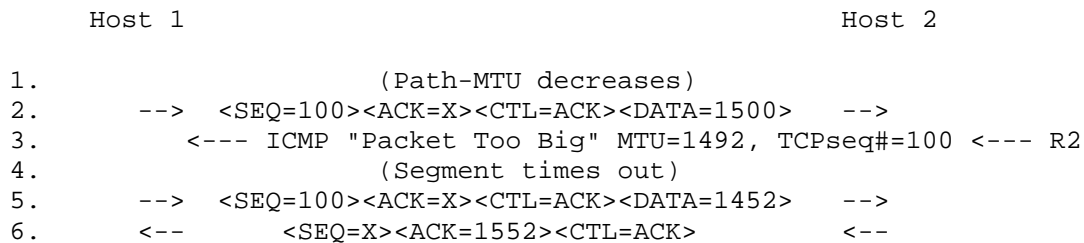
Figure 3: Operation during Path-MTU changes
