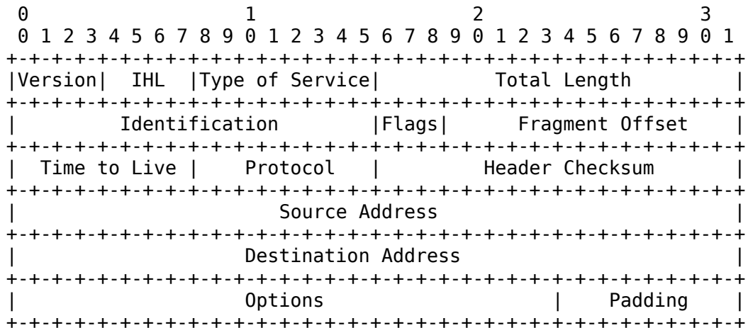
Figure 1: Internet Protocol header format
